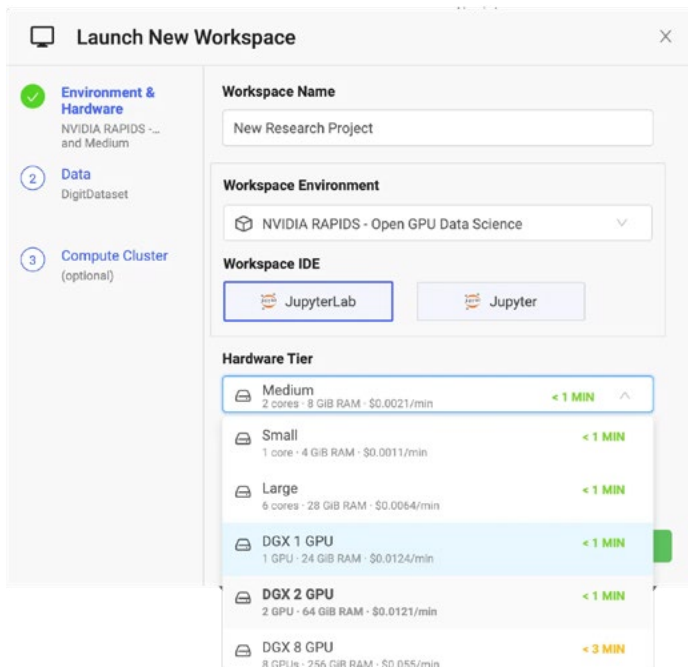
Figure 1: Domino users can launch on-demand workspaces with the latest NVIDIA GPUs, optimized with open-source and commercial data science tools.
